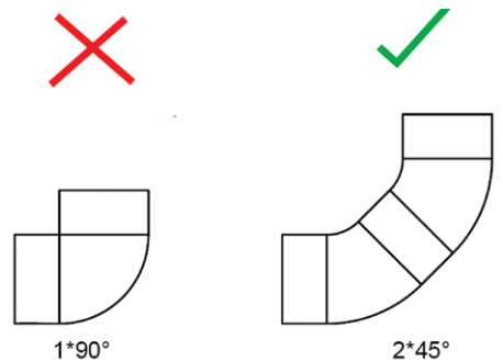
Incorrect and correct ways to install pipe bends
